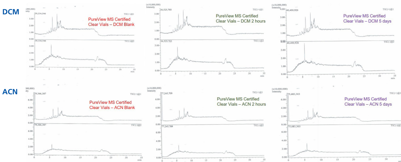
LC/MS (+) and (-) TIC scans of PureView MS Certified clear vials with ACN (blank, 2-hour extraction, 5-day extraction).
